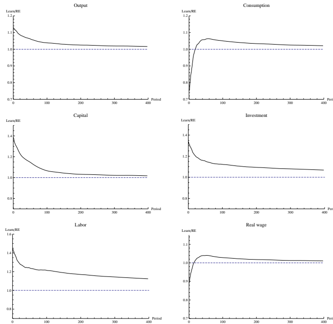
Figure 5: Volatility: Ratio of standard deviations under learning and RE.
