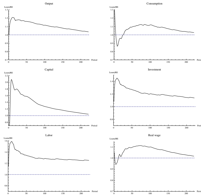
Figure 6: Percentage difference between learning and RE.
